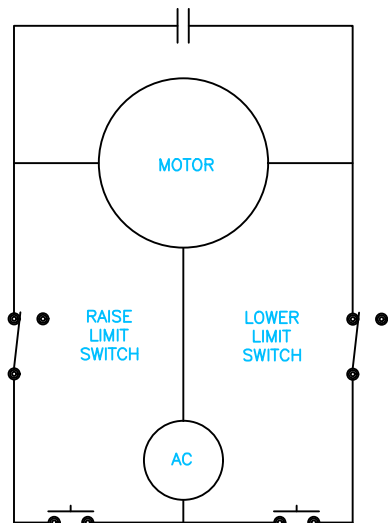
MOTOR CIRCUIT
