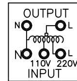
termination board INPUT:110/220V
